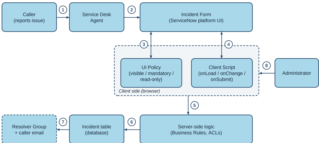
Figure 1: Architecture and data flow of the Incident form with UI Policy and Client Script
